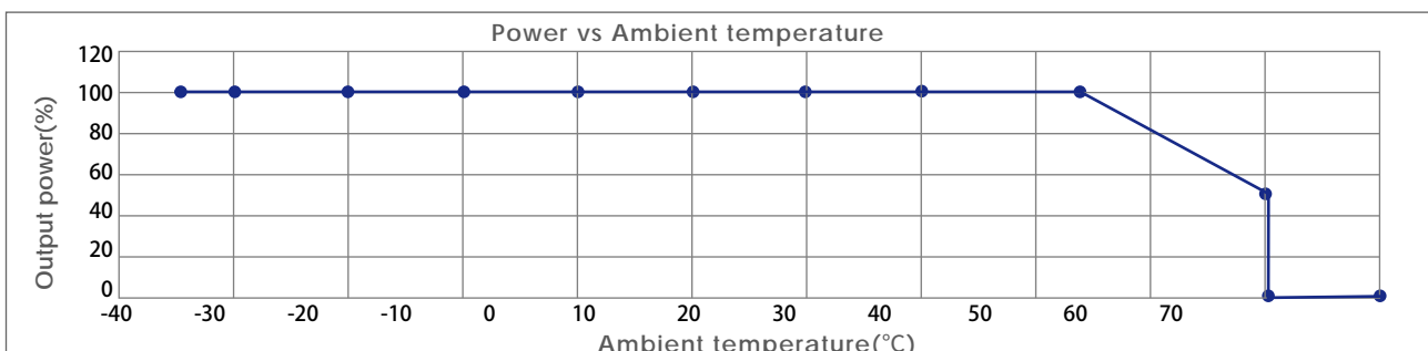
Power vs Ambient temperature curve
