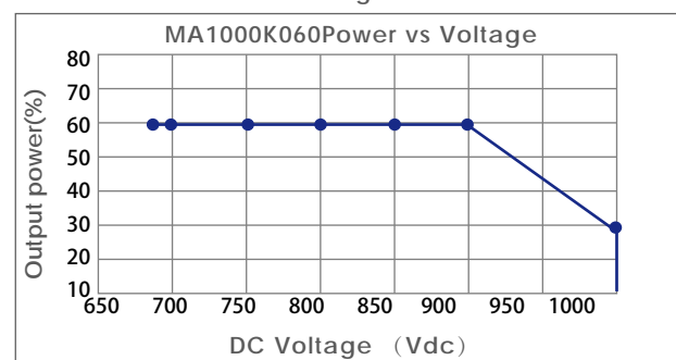
MA1000K060 Power vs Voltage curve
